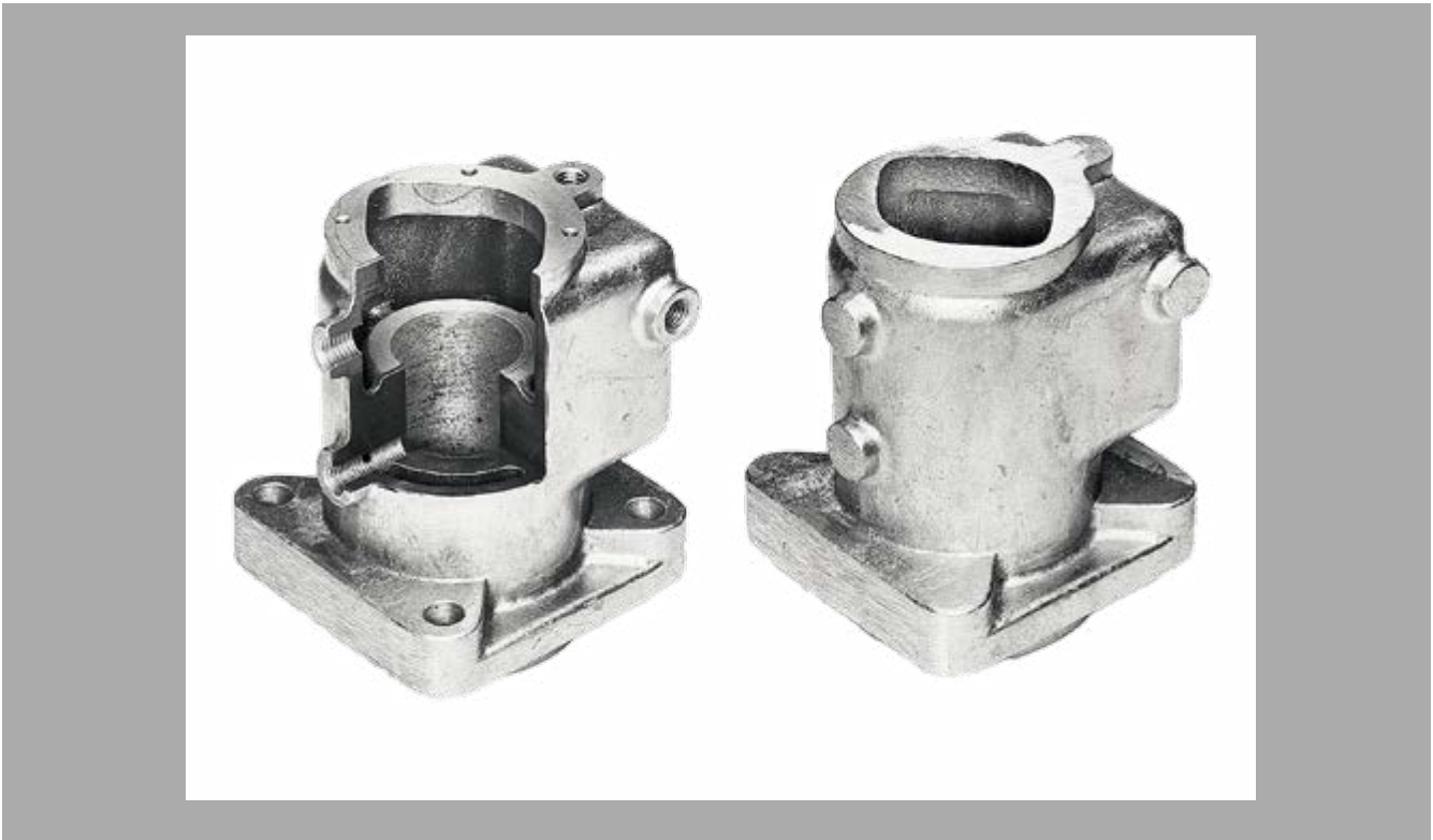
Machined (left) and unmachined (right) cast parts
