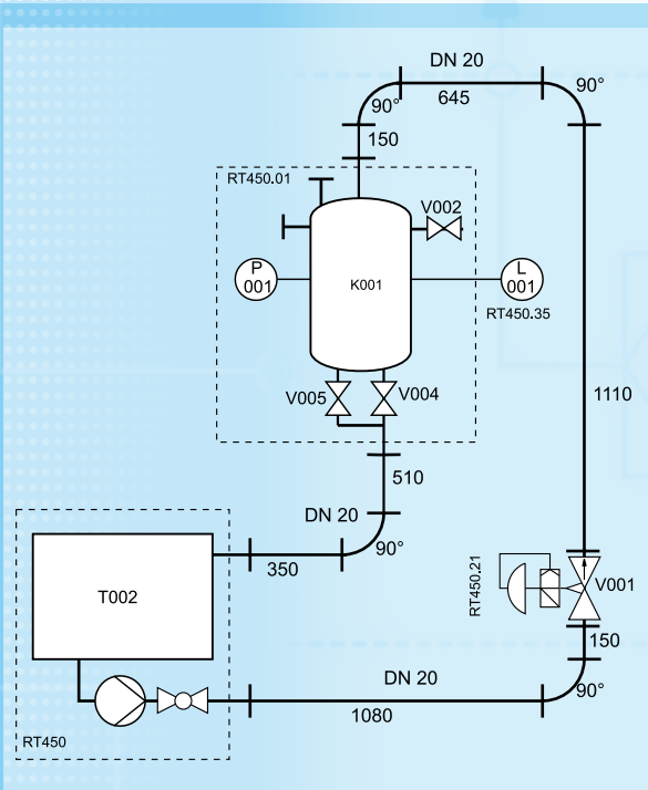
Pipework diagram for level control
