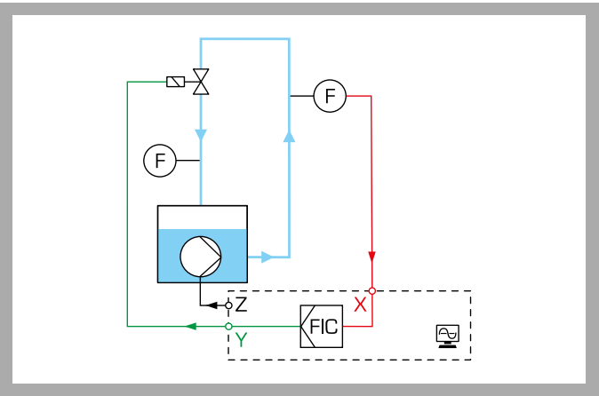
Process schematic
