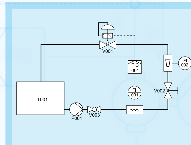
Flow control
