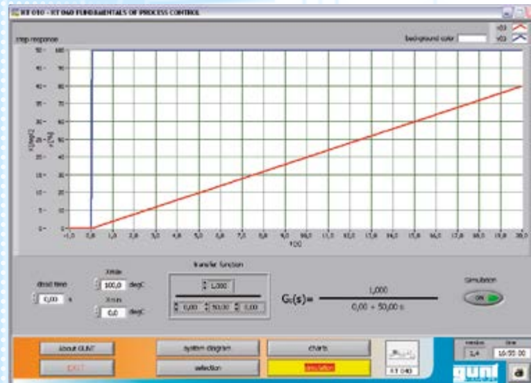
Integral behaviour
