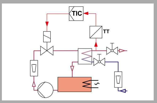
Process schematic
