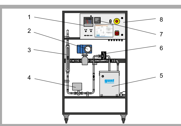
1 line recorder, 2 electromagnetic flow rate sensor, 3 rotameter, 4 control valve, 5 storage tank with pump, 6 ball valve with scale, 7 controller, 8 switch cabinet
