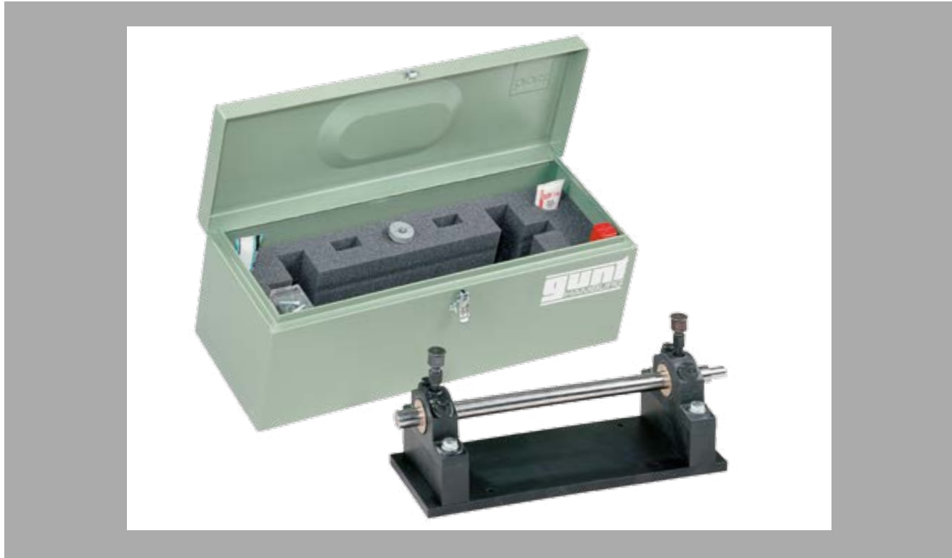
The illustration shows the tool box with parts set. A fully assembled journal bearing is shown in the foreground.
