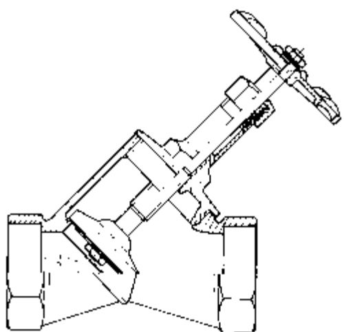
Sectional view of the HM 700.06 Angle Seat Valve
