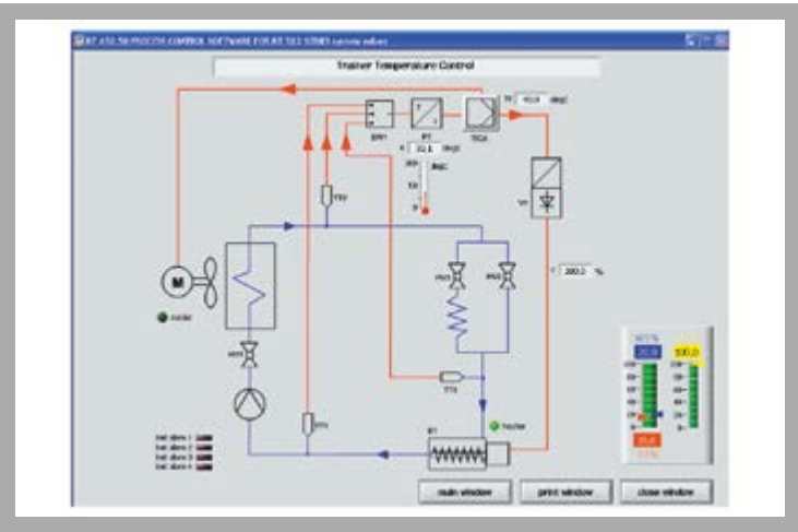
Process schematic for temperature control: reference variable W (setpoint) is settable directly; manipulating variable Y and controlled variable X (actual value) are displayed directly; controller can be accessed to change the parameters
