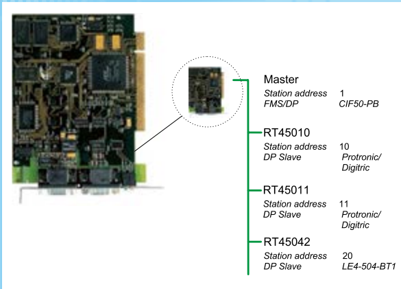
RT 450.40 is pre-set for two controllers and the PLC over Profibus. Changes can be made at any time.
