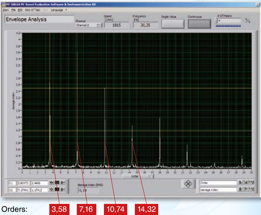
Screenshot of an envelope analysis showing outer race damage
