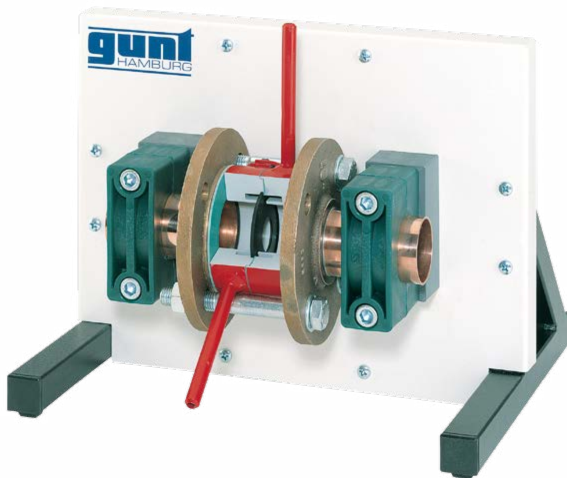
HM 700.01 Cutaway Model: Standard Orifice Plate
