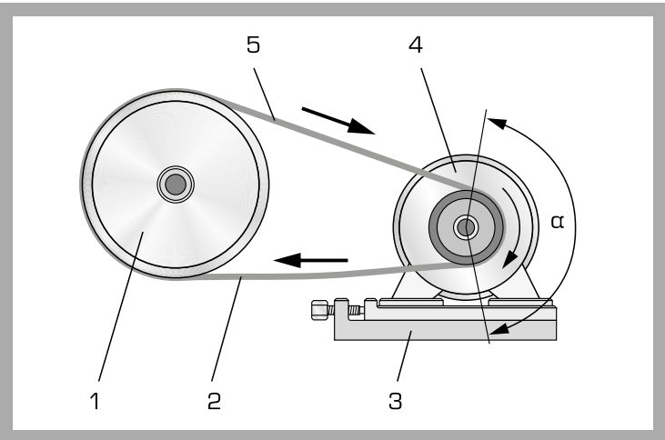
Mode of operation of a belt drive: 1 driven, 2 loose side, 3 slide rail with bolts, 4 drive, 5 load side, α angle of contact
