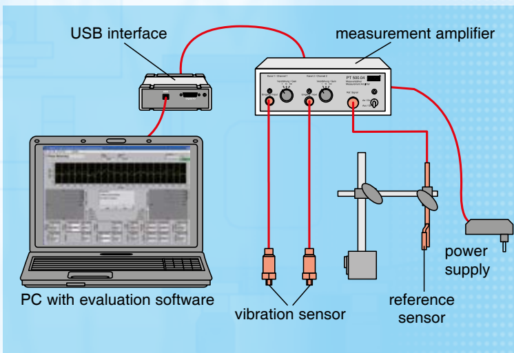
Measuring system set-up
