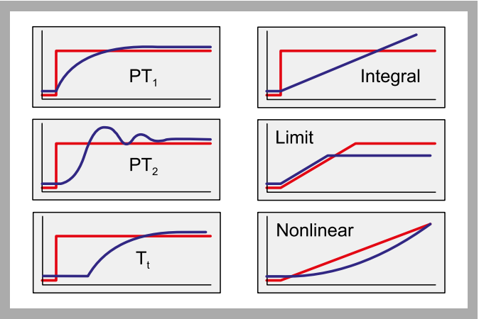
A wide range of controlled system characteristics can be simulated: PT 1 first order lag; PT 2 second order lag; T i time-delayed process
