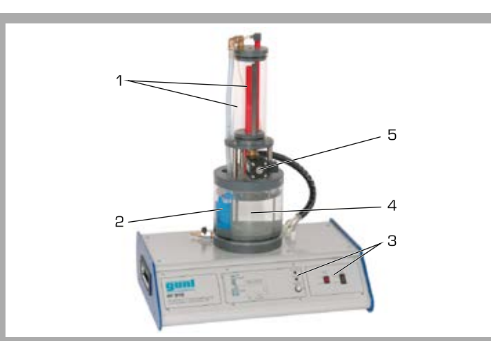
1 level-controlled tank with overflow, 2 pump, 3 displays and controls, 4 storage tank, 5 proportional valve
