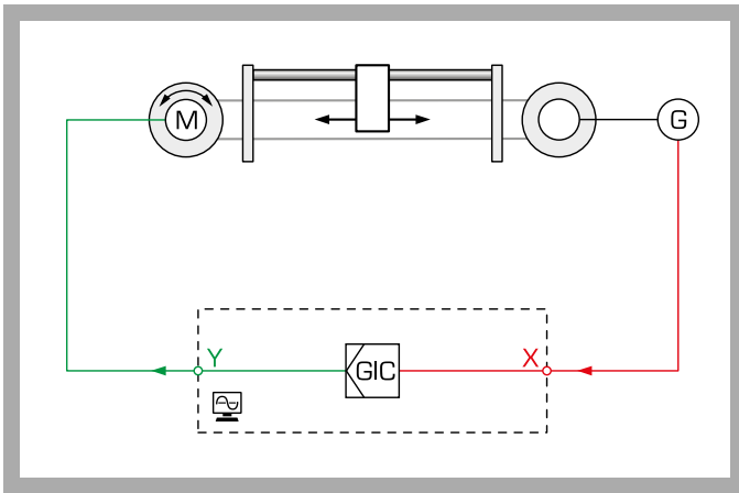
Process schematic
