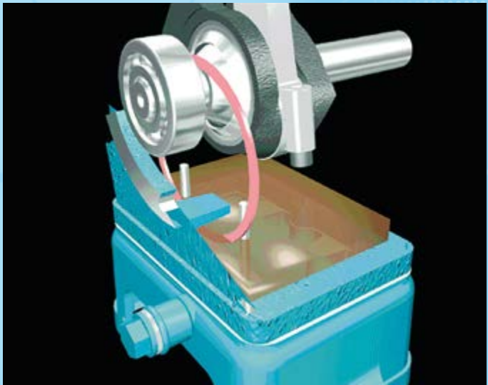
Crankcase, crankshaft, oil distribution ring
