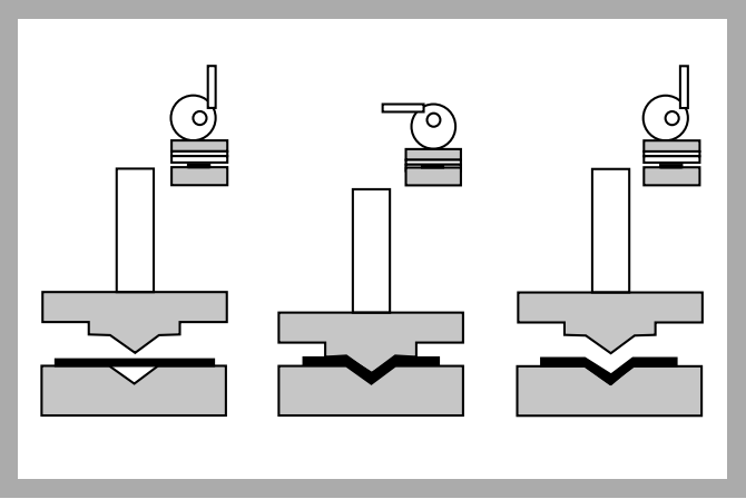
Bending process
