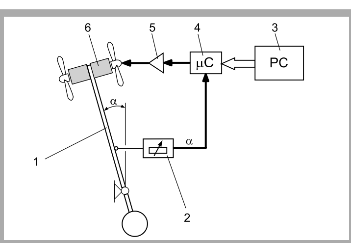
1 inverted pendulum, 2 pendulum inclination sensor, 3 PC with development software, 4 microcontroller, 5 amplifier, 6 drive motors with propellers
