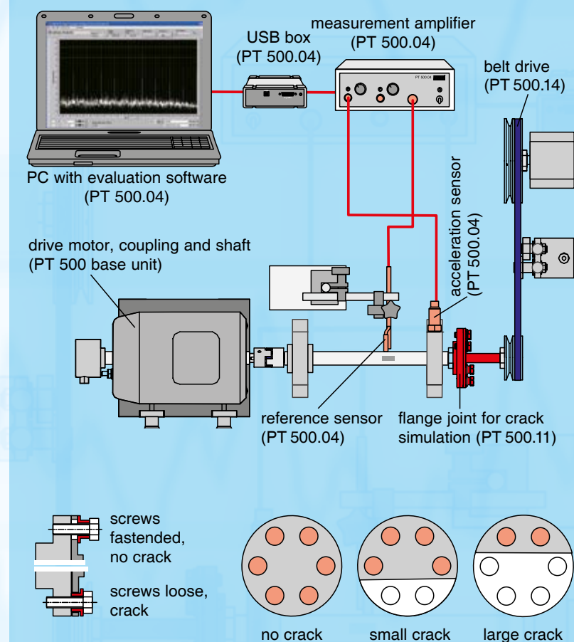
Simulation of a crack via a flange joint
