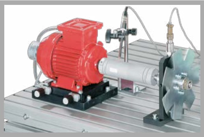
The illustration shows PT 500.18 together with PT 500 and PT 500.01.
