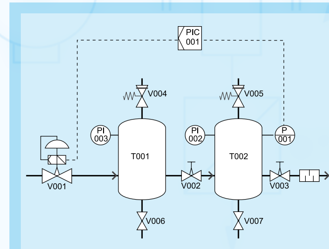
Pressure control
