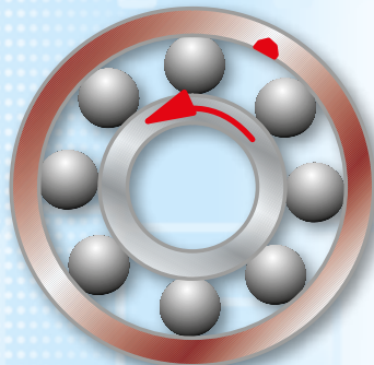
Bearing surface damage to the outer race, frequency 3,58 \Omega
