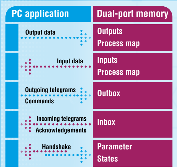
Data interchange between the application and the communications interface is run via a dual-port memory.
