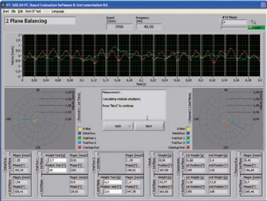
Screenshot: Balancing in two planes
