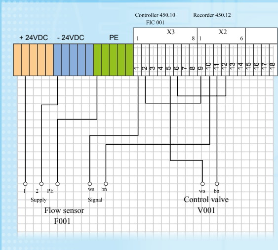
Plan of terminal connections for flow control
